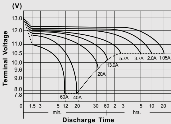
Discharge Characteristics
